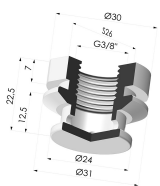
Detachable fitting female G3/8"
