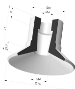
Flat Suction Cup Series 9, Ø 16 mm
