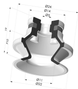
Bellows Suction Cup 1.5 folds Series 91, Ø 20 mm
