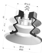
Bellows Suction Cup 2.5 folds Series 96B, Ø 30 mm
