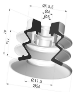
Bellows Suction Cup 2.5 folds Series 96C, Ø 25 mm
