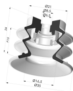
Bellows Suction Cup 2.5 folds Series 96C, Ø 35 mm
