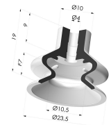
Bellows Suction Cup 1.5 folds Series 1, Ø 23 mm - With level on sealing lip Product reference: 1 23-- A SPD
