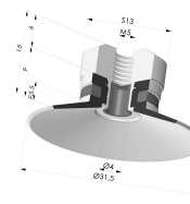
Flat Suction Cup Series 9, Ø 30 mm
