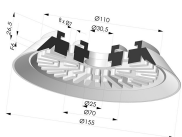
Flat Suction Cup Series 90, Ø 150 mm Product reference: 90 150-- A
