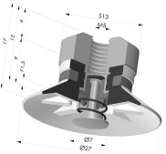
Flat Suction Cup Series 90, Ø 25 mm Product reference: 90 25-- FM5PAL
