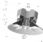
Flat Suction Cup Series 90, Ø 25 mm Product reference: 90 25-- FM5F
