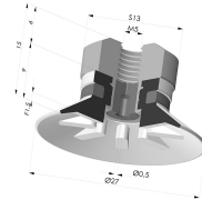
Flat Suction Cup Series 90, Ø 25 mm Product reference: 90 25-- FM5GIC
