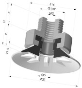
Flat Suction Cup Series 90, Ø 25 mm Product reference: 90 25-- 18
