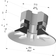
Flat Suction Cup Series 90, Ø 25 mm Product reference: 90 25-- FM5
