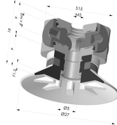
Flat Suction Cup Series 90, Ø 25 mm Product reference: 90 25-- FM5BD
