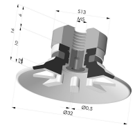
Flat Suction Cup Series 90, Ø 30 mm
