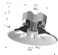
Flat Suction Cup Series 90, Ø 30 mm Product reference: 90 30-- FM5GIC
