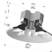
Flat Suction Cup Series 90, Ø 30 mm Product reference: 90 30-- FM5F
