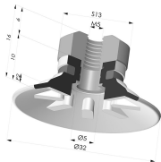
Flat Suction Cup Series 90, Ø 30 mm Product reference: 90 30-- FM5
