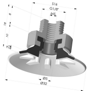
Flat Suction Cup Series 90, Ø 30 mm Product reference: 90 30-- 18
