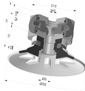
Flat Suction Cup Series 90, Ø 30 mm
