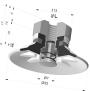
Flat Suction Cup Series 90, Ø 30 mm
