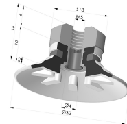
Flat Suction Cup Series 90, Ø 30 mm
