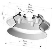
Bellows Suction Cup 1.5 folds Series 91, Ø 110 mm
