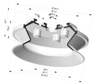
Bellows Suction Cup 1.5 folds Series 91, Ø 150 mm
