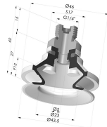
Bellows Suction Cup 1.5 folds Series 91, Ø 40 mm Product reference: 91 40-- 14D-2-F
