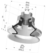
Bellows Suction Cup 1.5 folds Series 91, Ø 40 mm Product reference: 91 40-- 18
