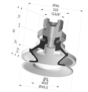
Bellows Suction Cup 1.5 folds Series 91, Ø 40 mm Product reference: 91 40-- 38D-2-F
