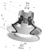
Bellows Suction Cup 1.5 folds Series 91, Ø 40 mm Product reference: 91 40-- 18D-2-GIC
