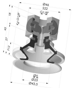
Bellows Suction Cup 1.5 folds Series 91, Ø 40 mm Product reference: 91 40-- 18D-3-BD
