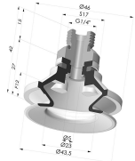
Bellows Suction Cup 1.5 folds Series 91, Ø 40 mm Product reference: 91 40-- 14D-2
