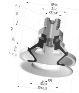
Bellows Suction Cup 1.5 folds Series 91, Ø 40 mm Product reference: 91 40-- 14D-2-GIC
