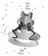
Bellows Suction Cup 1.5 folds Series 91, Ø 40 mm Product reference: 91 40-- 38D-2-GIC
