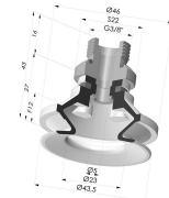
Bellows Suction Cup 1.5 folds Series 91, Ø 40 mm Product reference: 91 40-- 38D-2
