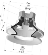
Bellows Suction Cup 1.5 folds Series 91, Ø 40 mm Product reference: 91 40-- 18D-2-F
