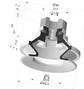
Bellows Suction Cup 1.5 folds Series 91, Ø 40 mm Product reference: 91 40-- 18D-2
