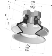
Bellows Suction Cup 1.5 folds Series 91, Ø 50 mm
