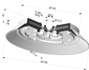
Flat suction cup series PFG, Ø 198 mm
