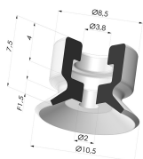
Flat suction cup series PFG Ø 10.5 mm
