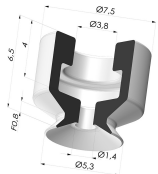
Flat suction cup series PFG Ø 5.3 mm
